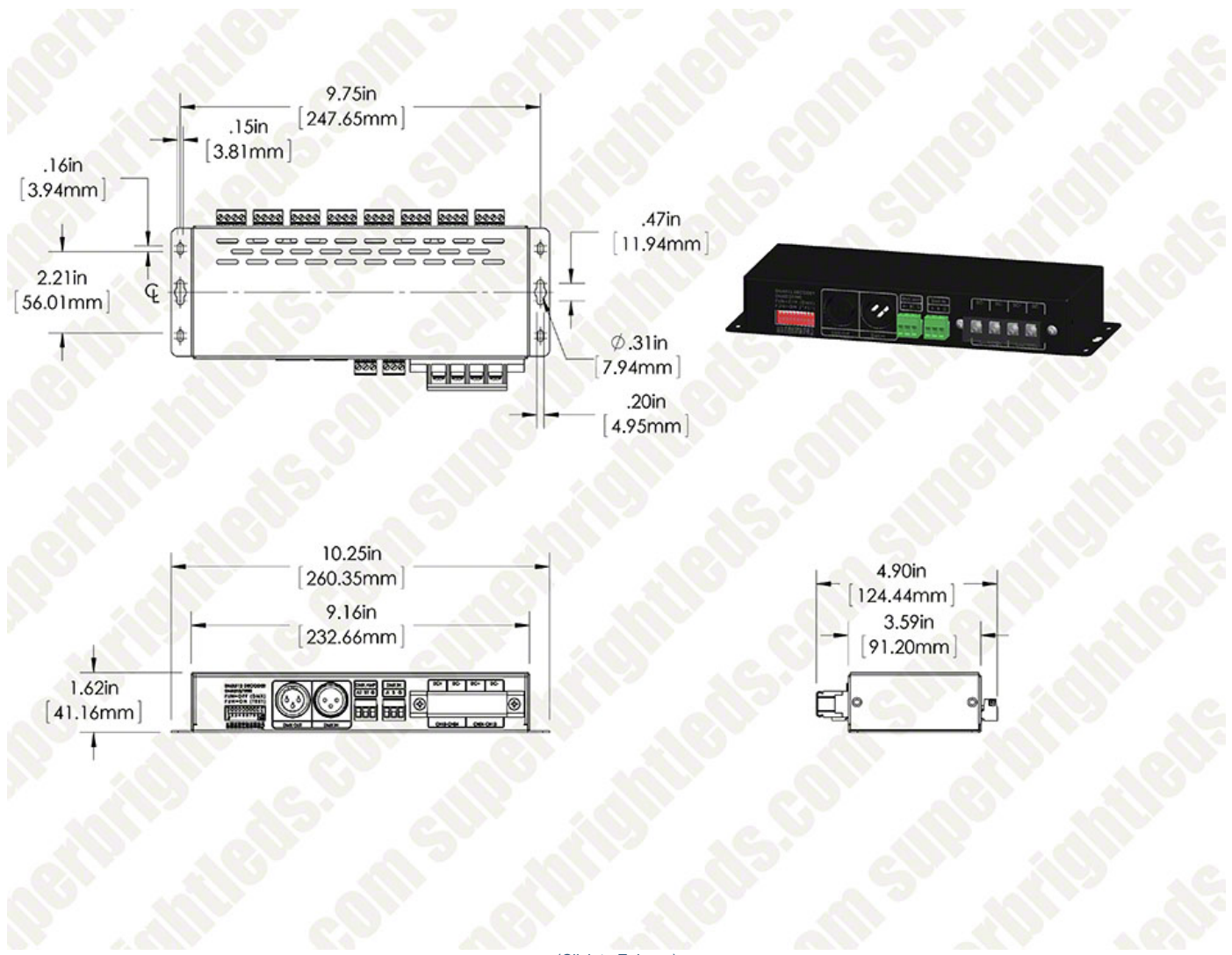
DMX-24CH-LV - DMX-24CH-LV 24 Channel LED DMX Controller/Decoder
